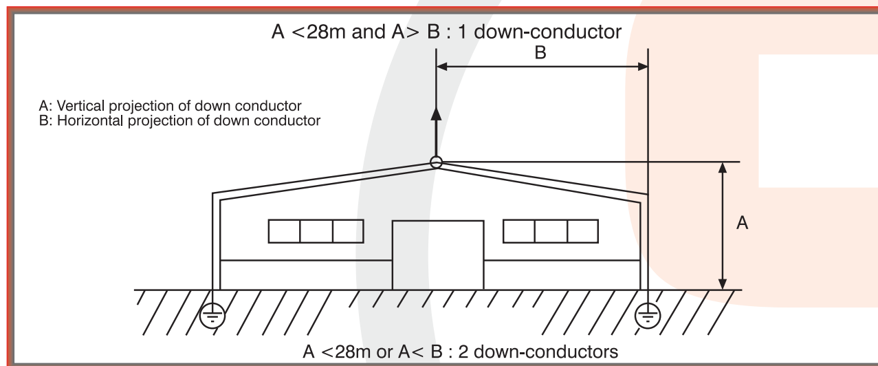
(Figure 1) - Number of down-conductors
